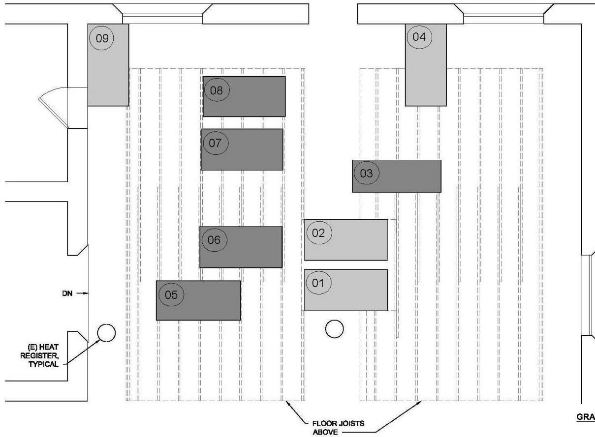
2 A-1 (E) BELOW FINISHED FLOOR PLAN SCALE: 1/4" = 1'-0" NORTH
